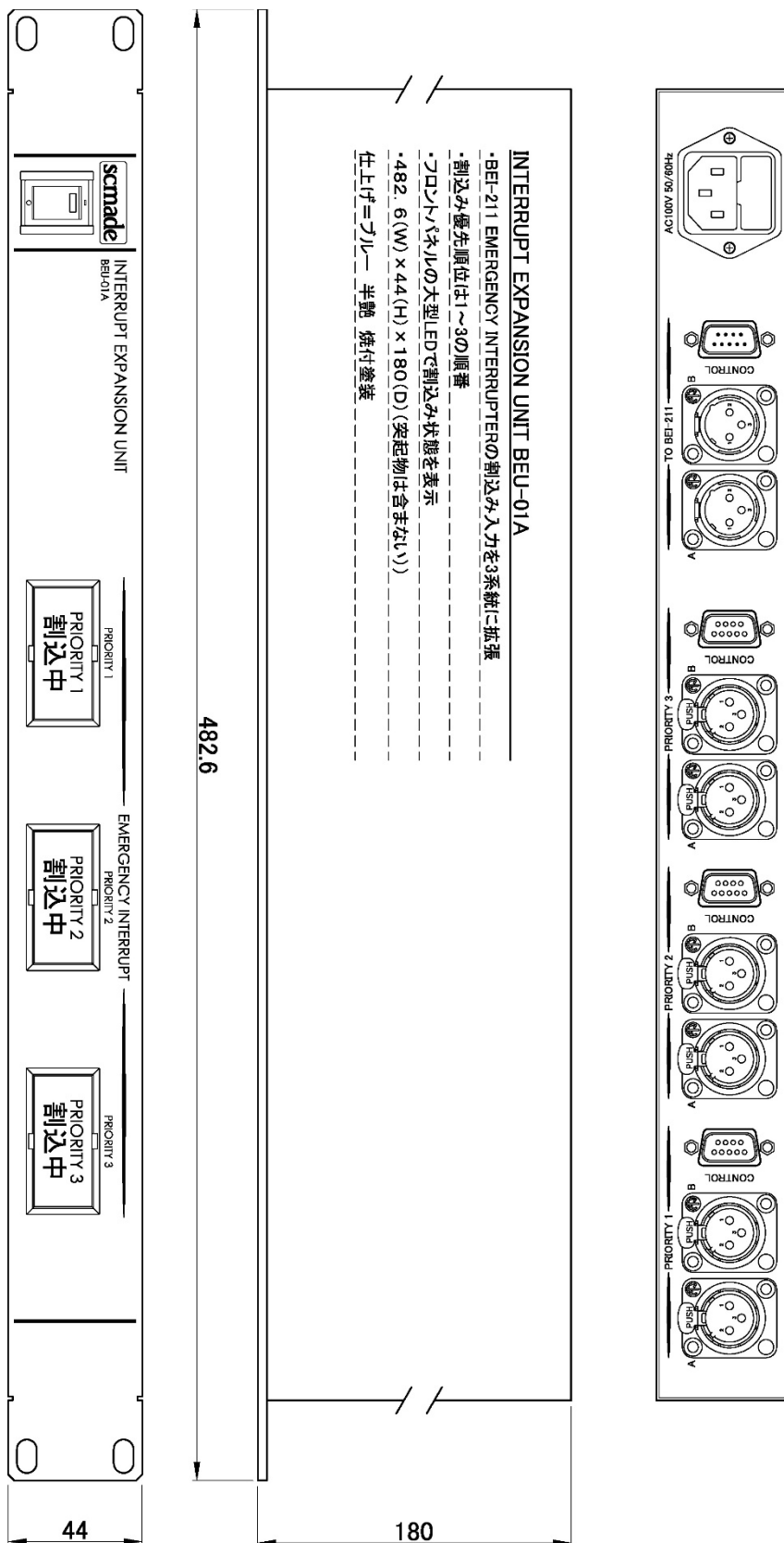
BEU-01A Expansion Unit
